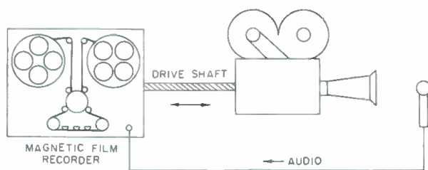
Figure 2. Mechanical interlock.
