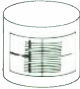
Figure 2. Head face showing area to which to apply silver paint. Avoid getting paint on the gap, shown by thin vertical line down the middle.
